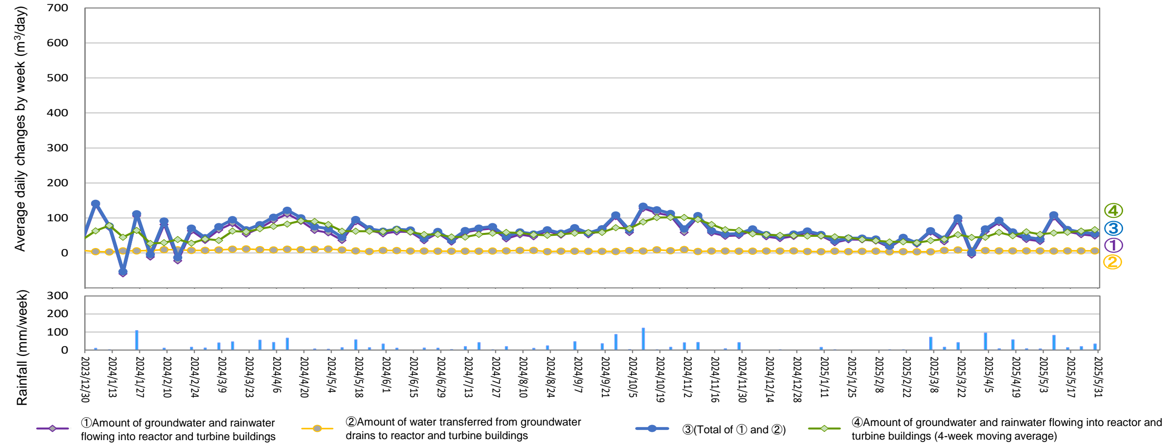
Amount of water transferred from groundwater drains to reactor and turbine buildings (From May 22, 2025 to May 28, 2025)
