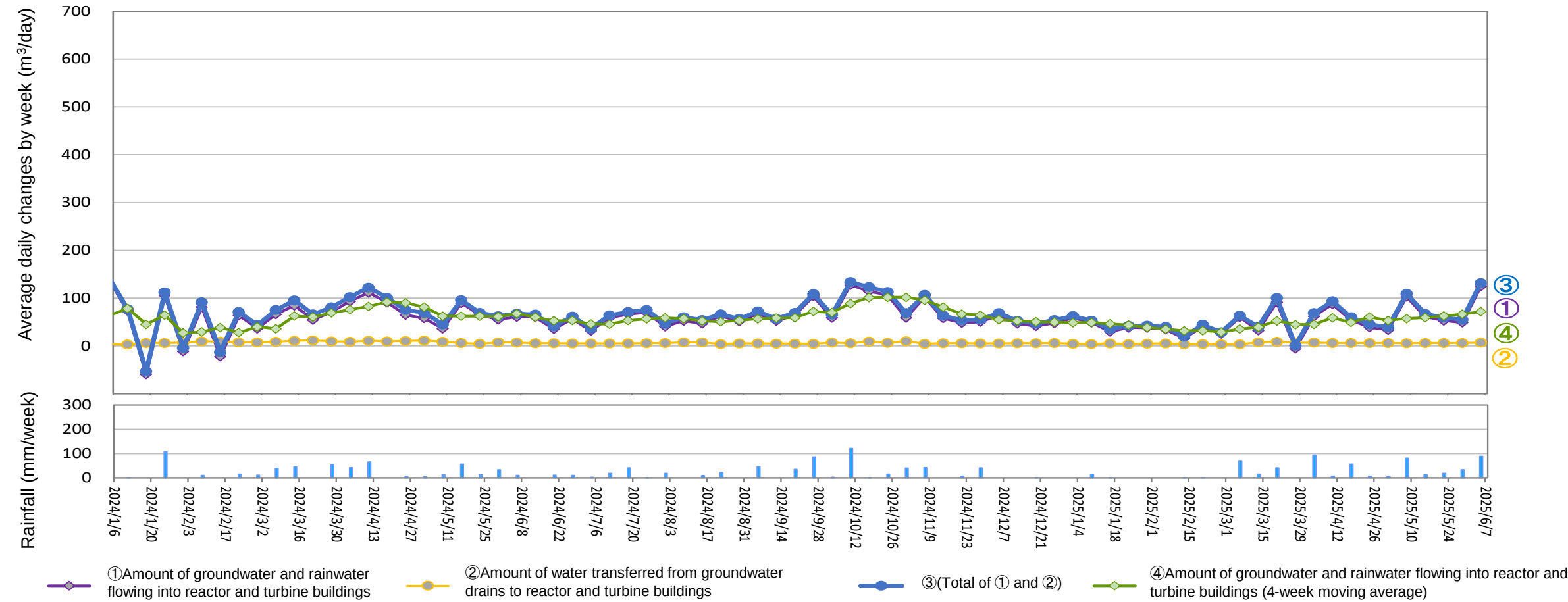
Amount of water transferred from groundwater drains to reactor and turbine buildings (From May 29, 2025 to June 4, 2025)
