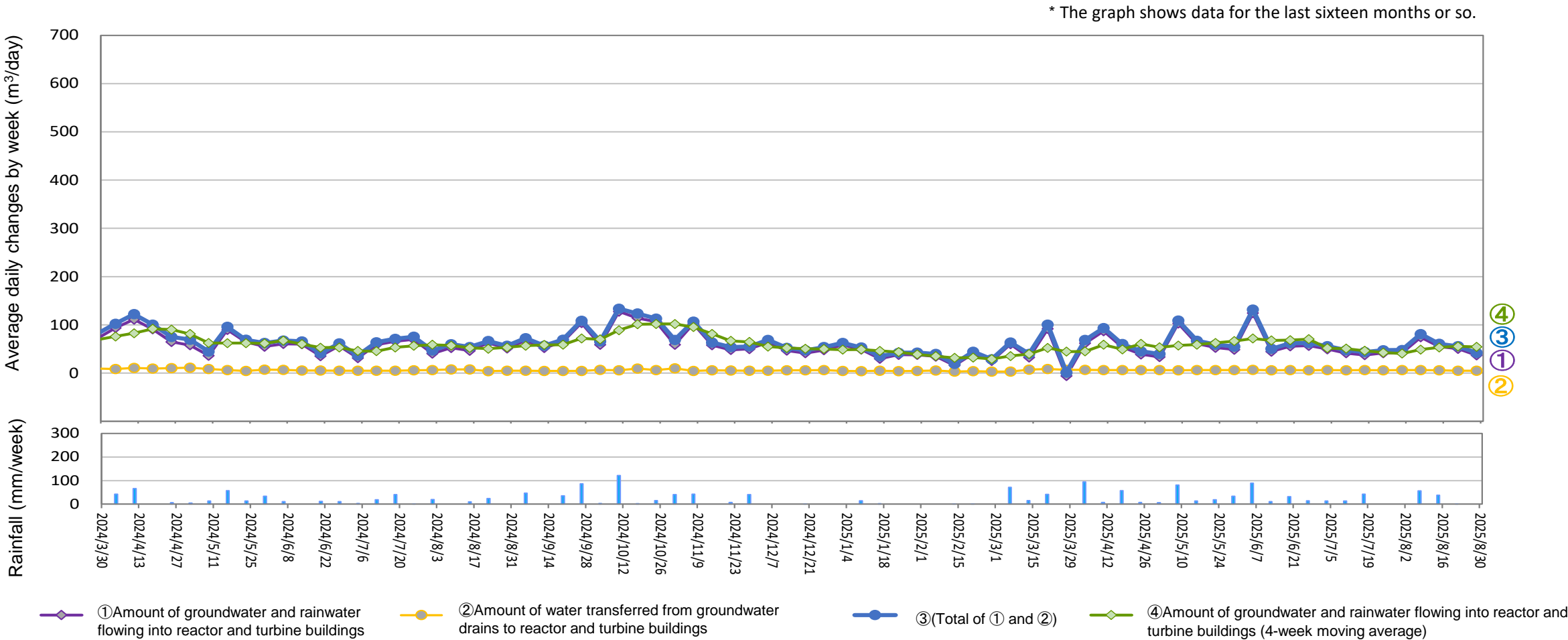
Amount of water transferred from groundwater drains to reactor and turbine buildings (From August 21, 2025 to August 27, 2025)
