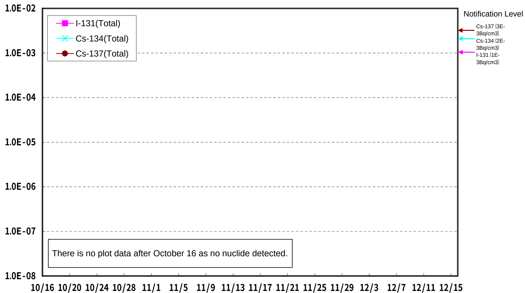
(Reference) Fukushima Daini MP-1 Results of Dust Nuclide Analysis (Bq/cm 3 )
